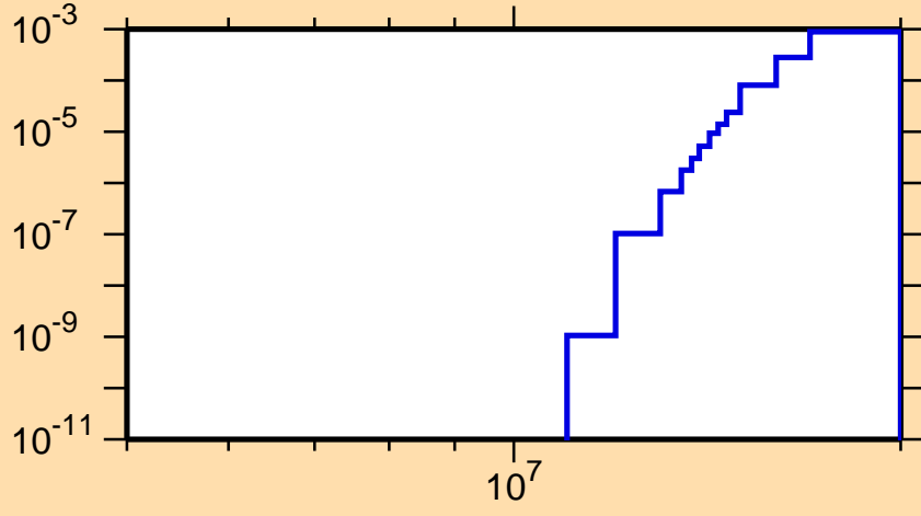
\sigma vs. E for ^{179}\text{Tm}(n,np)
