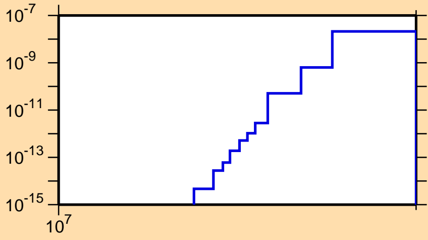
\sigma vs. E for ^{179}\text{Tm}(n,2n\alpha)
