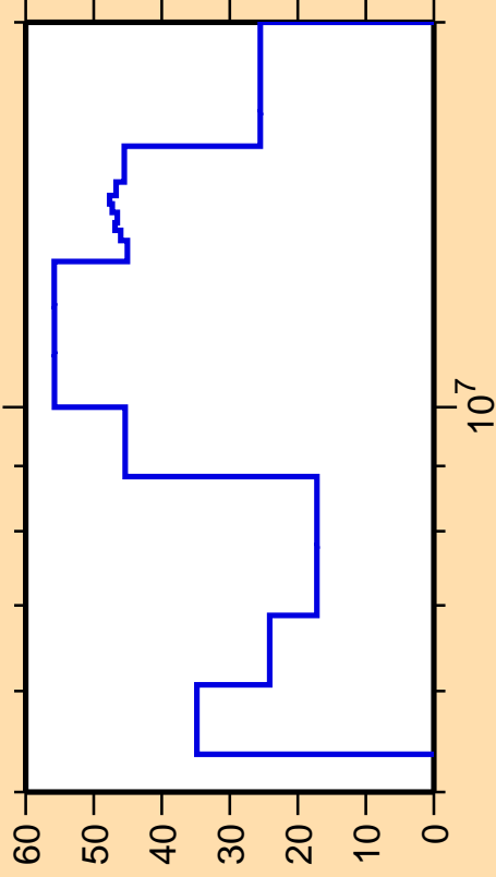
\Delta\sigma/\sigma vs. E for ^{179}\text{Tm}(n,2n)
