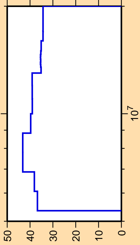
\Delta\sigma/\sigma vs. E for ^{179}\text{Tm}(n,n_1)
