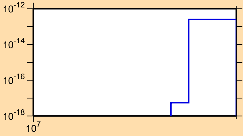
\sigma vs. E for ^{179}\text{Tm}(n,3n\alpha)
