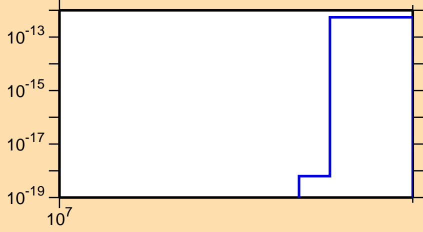
\sigma vs. E for ^{179}\text{Tm} (mt 11)
