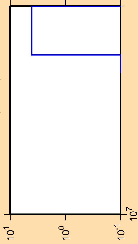
\Delta\sigma/\sigma vs. E for ^{179}\text{Tm} (mt 11)
