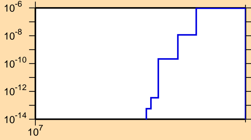
\sigma vs. E for ^{179}\text{Tm}(n,nd)
