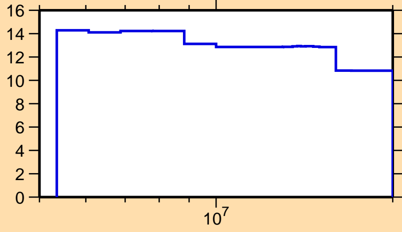
\Delta\sigma/\sigma vs. E for ^{179}\text{Tm}(n,\text{nonel.})
