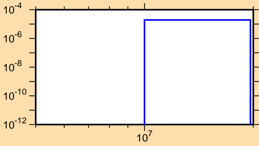
\sigma vs. E for ^{179}\text{Tm}(n,t)
