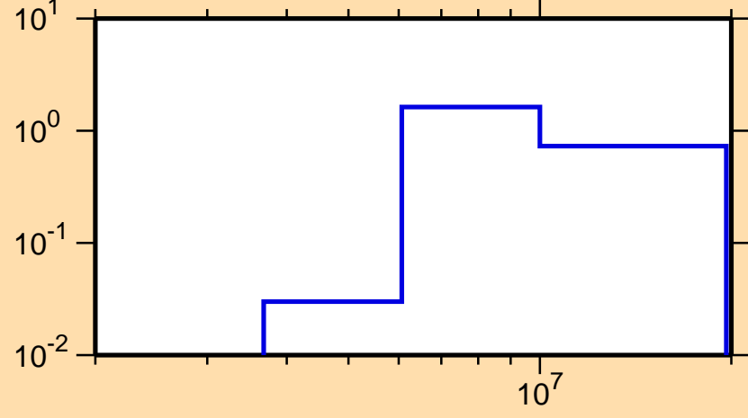
\sigma vs. E for ^{179}\text{Tm}(n,2n)
