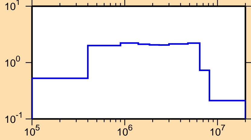
\sigma vs. E for ^{179}\text{Tm}(n,\text{inel.})
