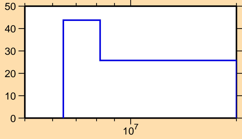
\Delta\sigma/\sigma vs. E for ^{179}\text{Tm}(n,ncont.)
