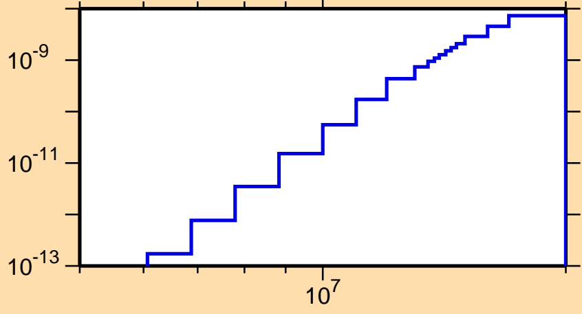
\sigma vs. E for ^{227}\text{U}(n,p\alpha)
