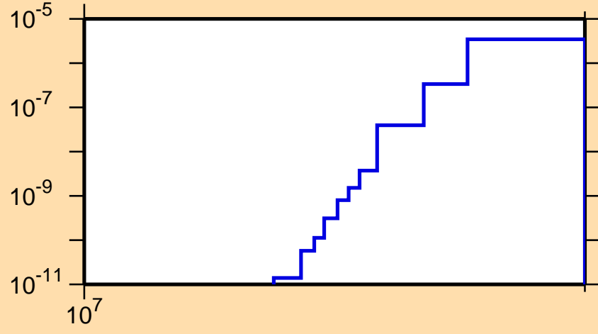
\sigma vs. E for ^{227}\text{U}(n,nd)
