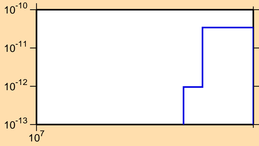
\sigma vs. E for ^{227}\text{U} (mt 34)
