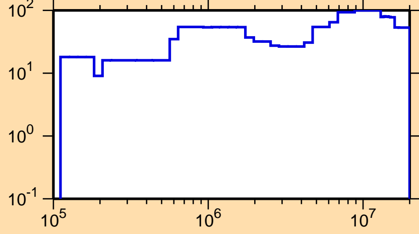
\Delta\sigma/\sigma vs. E for ^{227}\text{U}(n,\text{el.})
