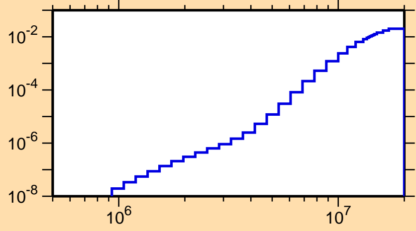
\sigma vs. E for ^{227}\text{U}(n,p)
