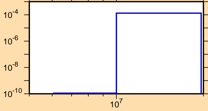
\sigma vs. E for ^{227}\text{U}(n,t)
