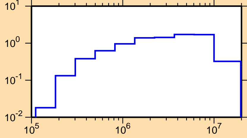
\sigma vs. E for ^{227}\text{U}(n,\text{inel.})
