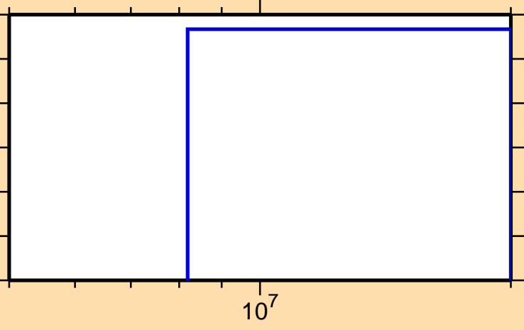
\sigma vs. E for ^{227}\text{U}(n,\text{He3})
