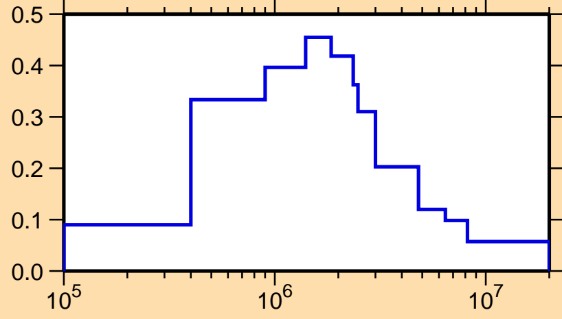
\sigma vs. E for ^{227}\text{U}(n,n_1)
