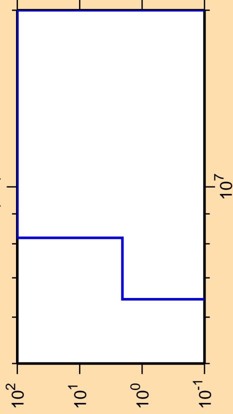
\Delta\sigma/\sigma vs. E for ^{227}\text{U}(n,t)
