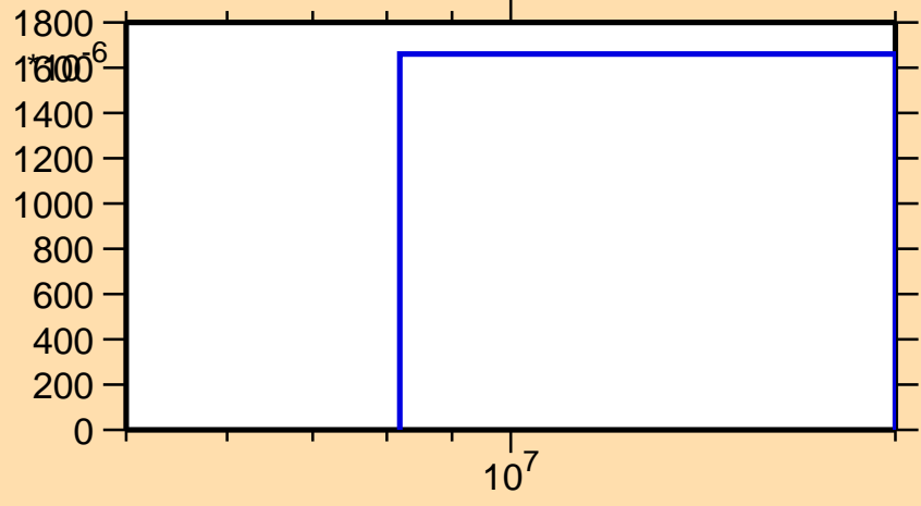
\sigma vs. E for ^{227}\text{U}(n,3n\alpha)
