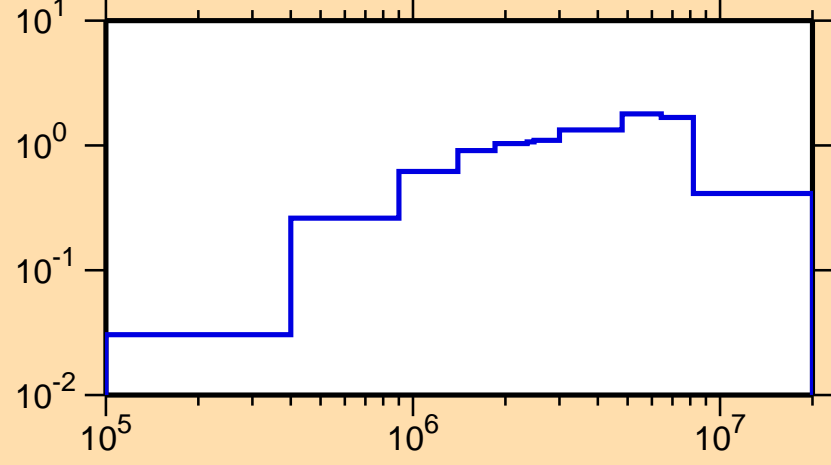
\sigma vs. E for ^{227}\text{U}(n,n\text{cont.})
