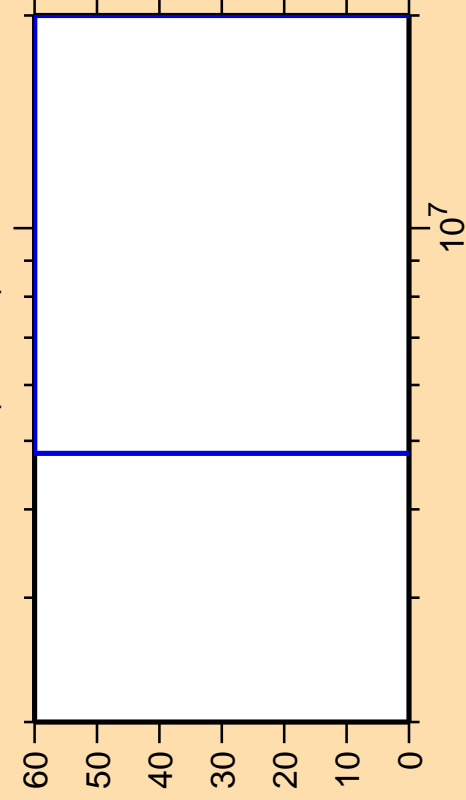
\Delta\sigma/\sigma vs. E for ^{227}\text{U}(n,2n\alpha)
