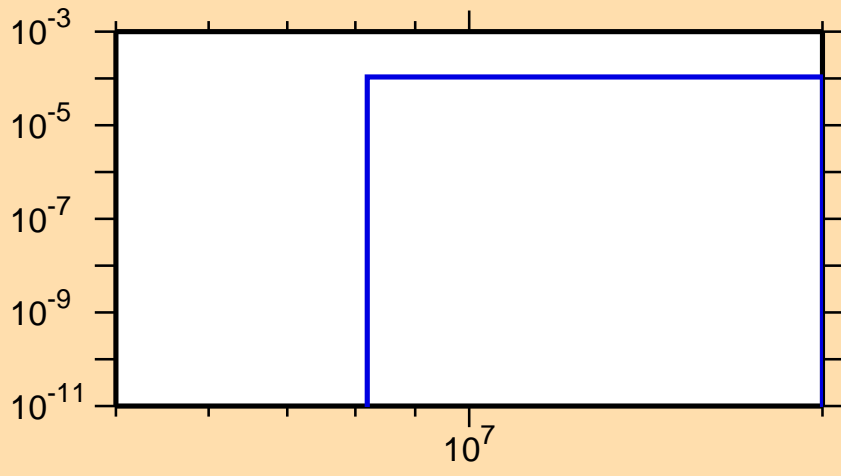
\sigma vs. E for ^{227}\text{U}(n,t)
