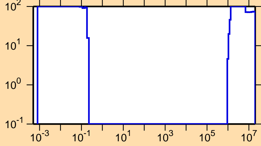
\Delta\sigma/\sigma vs. E for ^{229}\text{U}(n,p)
