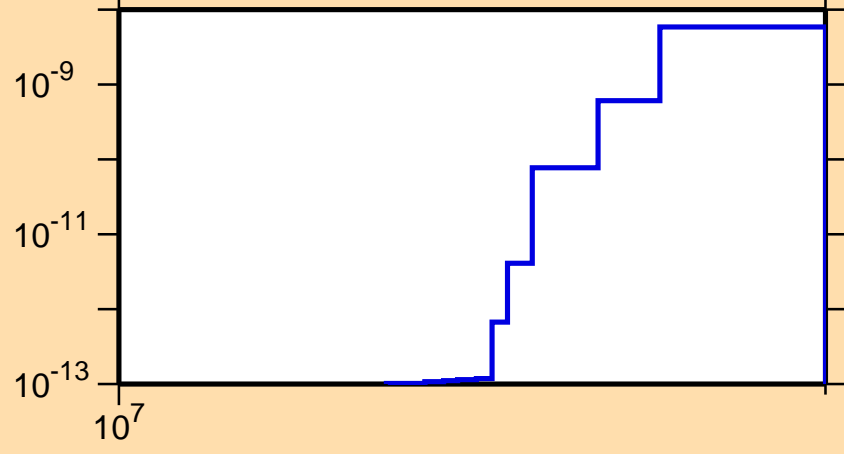
\sigma vs. E for ^{229}\text{U}(n,3n\alpha)
