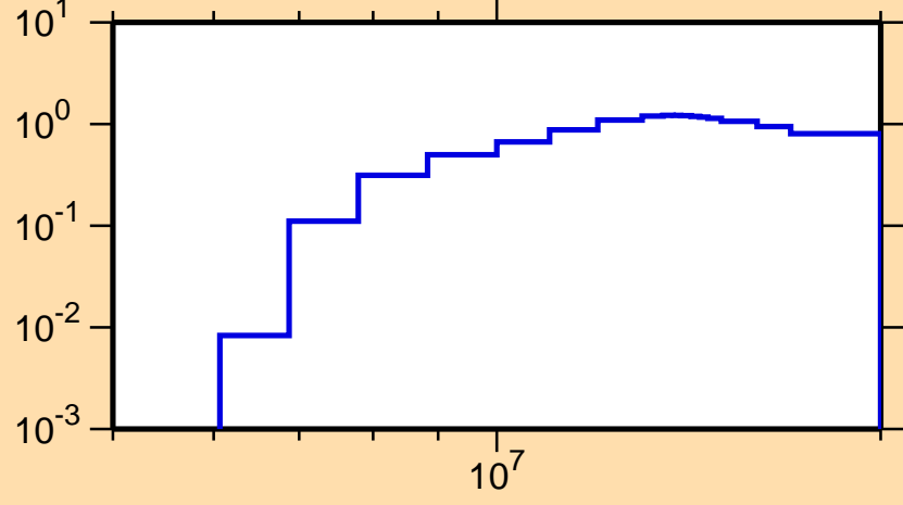
\sigma vs. E for ^{229}\text{U}(n,2n)
