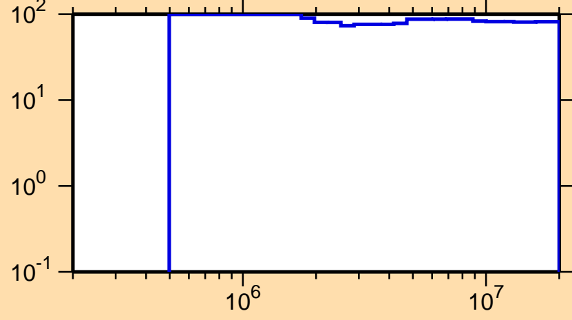
\Delta\sigma/\sigma vs. E for ^{229}\text{U}(n,ncont.)
