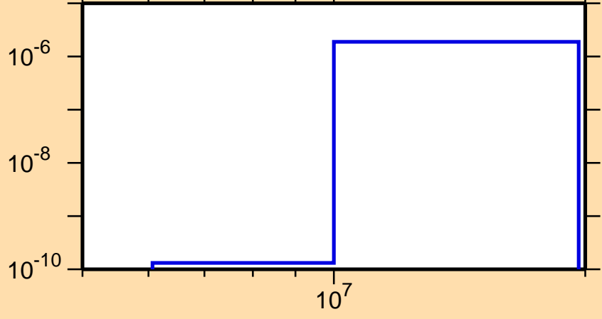
\sigma vs. E for ^{229}\text{U}(n,2n\alpha)
