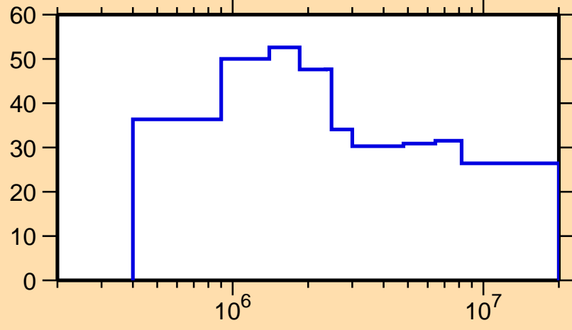
\Delta\sigma/\sigma vs. E for ^{229}\text{U}(n,n\text{onel.})
