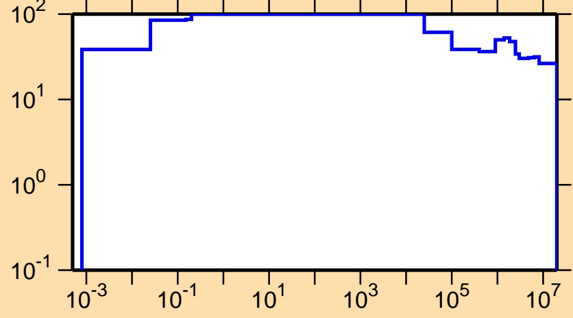
\Delta\sigma/\sigma vs. E for ^{229}\text{U}(n,\text{nonel.})
