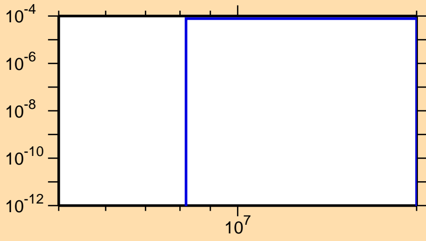
\sigma vs. E for ^{229}\text{U}(n,t)
