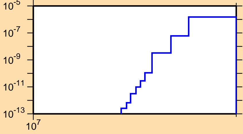
\sigma vs. E for ^{235}\text{U}(n,nd)
