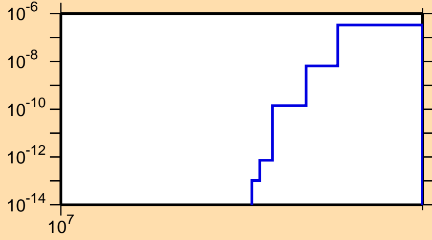
\sigma vs. E for ^{235}\text{U}(n,2np)
