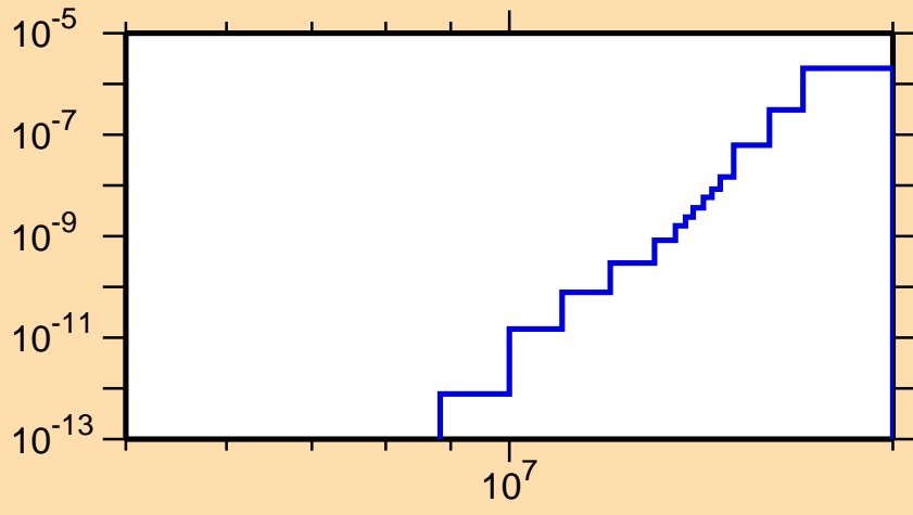
\sigma vs. E for ^{235}\text{U}(n,2n\alpha)
