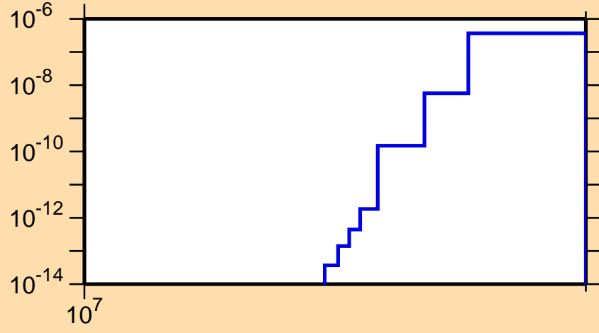
\sigma vs. E for ^{235}\text{U}(n,nt)
