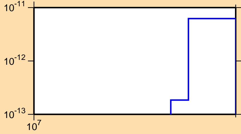
\sigma vs. E for ^{235}\text{U}(n,3n\alpha)
