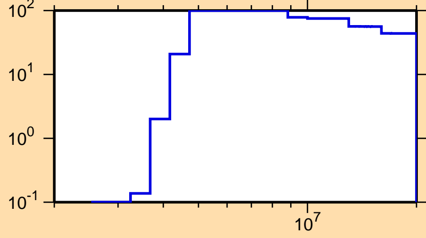
\Delta\sigma/\sigma vs. E for ^{235}\text{U}(n,p)
