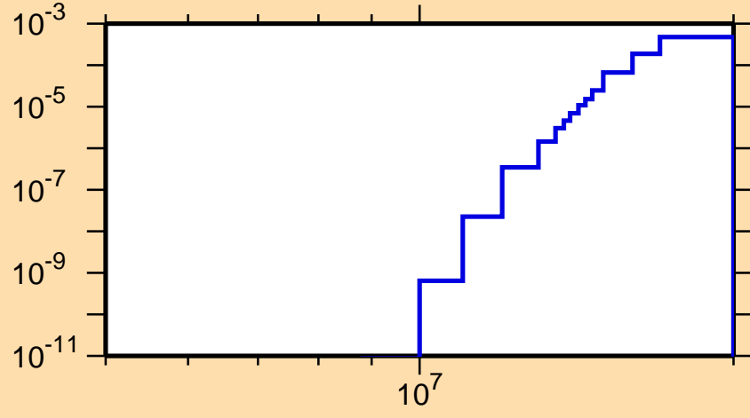
\sigma vs. E for ^{235}\text{U}(n,t)
