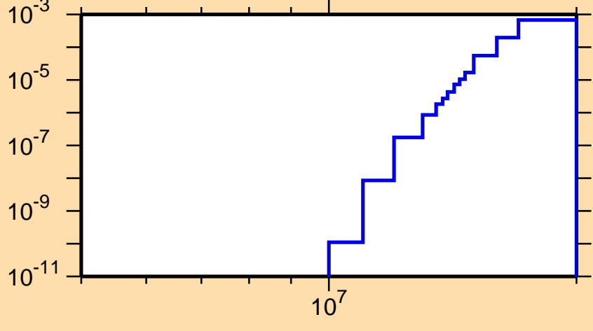
\sigma vs. E for ^{235}\text{U}(n,np)
