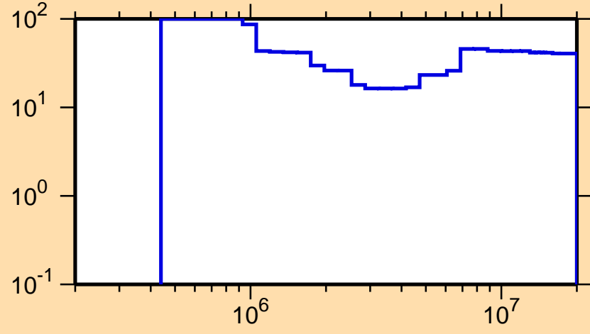
\Delta\sigma/\sigma vs. E for ^{235}\text{U}(n,ncont.)
