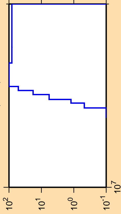
\Delta\sigma/\sigma vs. E for ^{235}\text{U}(n,nd)
