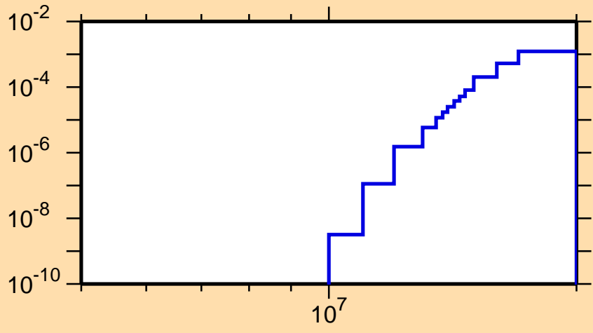
\sigma vs. E for ^{235}\text{U}(n,d)
