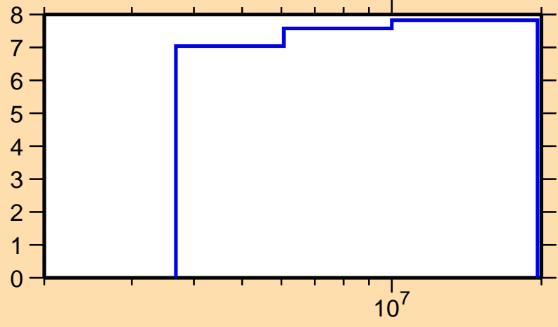
\Delta\sigma/\sigma vs. E for ^{235}\text{U}(n,\text{nonel.})
