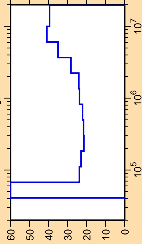
\Delta\sigma/\sigma vs. E for ^{235}\text{U}(n,n_3)
