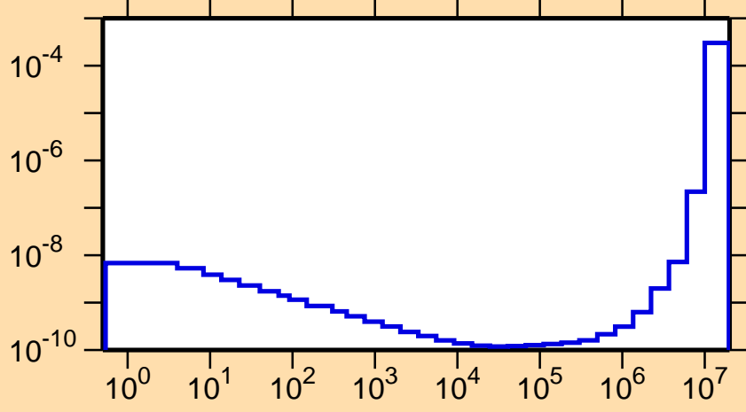
\sigma vs. E for ^{235}\text{U}(n,\alpha)
