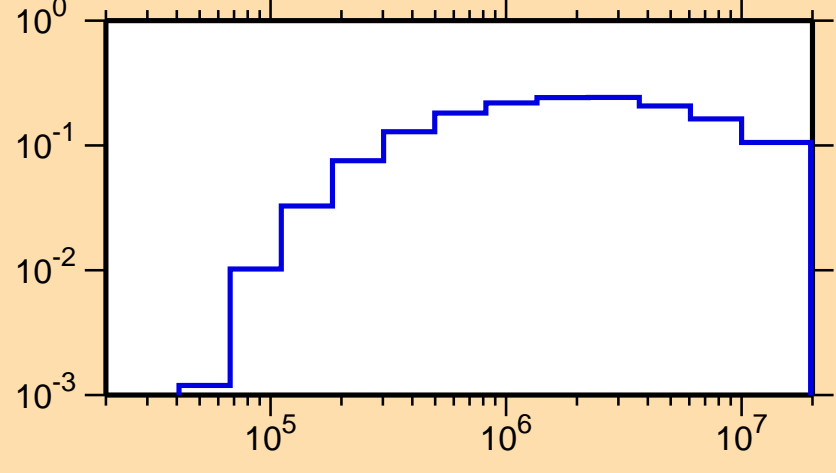
\sigma vs. E for ^{235}\text{U}(n,n_3)
