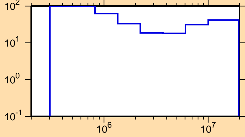
\Delta\sigma/\sigma vs. E for ^{235}\text{U}(n,ncont.)
