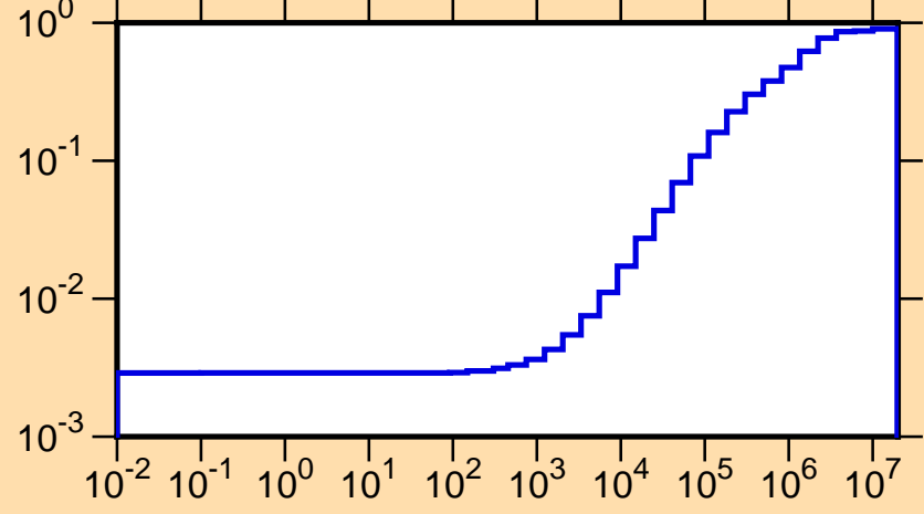
\mu vs. E for ^{236}\text{U}(\text{mt251})
