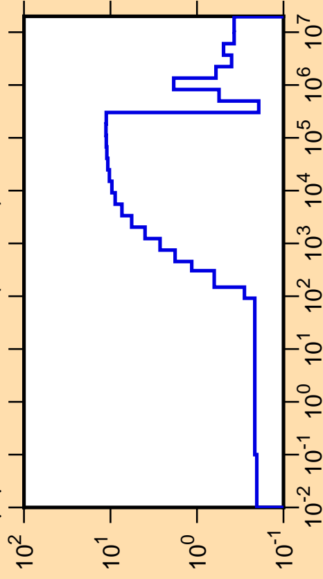
\Delta\mu/\mu vs. E for ^{236}\text{U}(\text{mt251})
