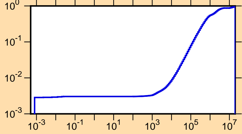
\mu vs. E for ^{237}\text{U}(\text{mt251})
