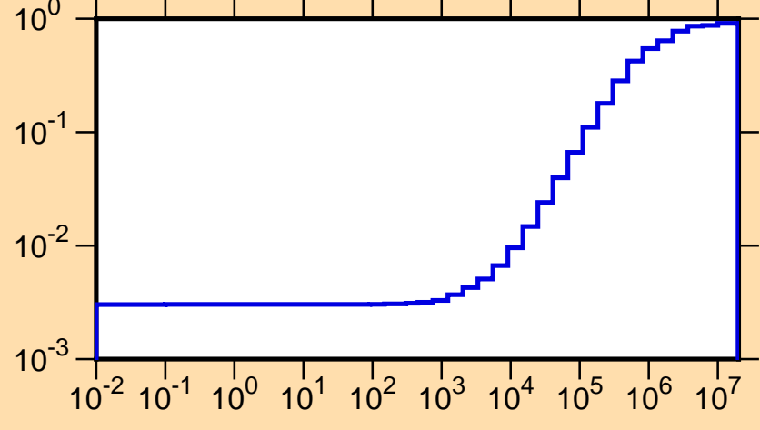
\mu vs. E for ^{237}\text{U}(\text{mt251})
