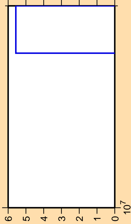
\Delta\sigma/\sigma vs. E for ^{240}\text{U}(n,3n\alpha)
