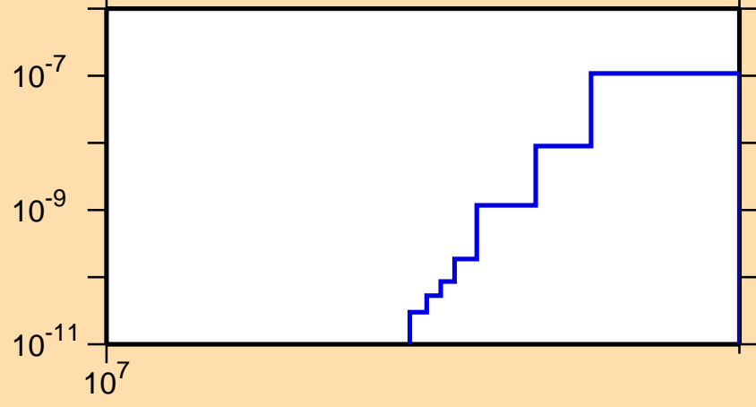
\sigma vs. E for ^{240}\text{U}(n,2n\alpha)
