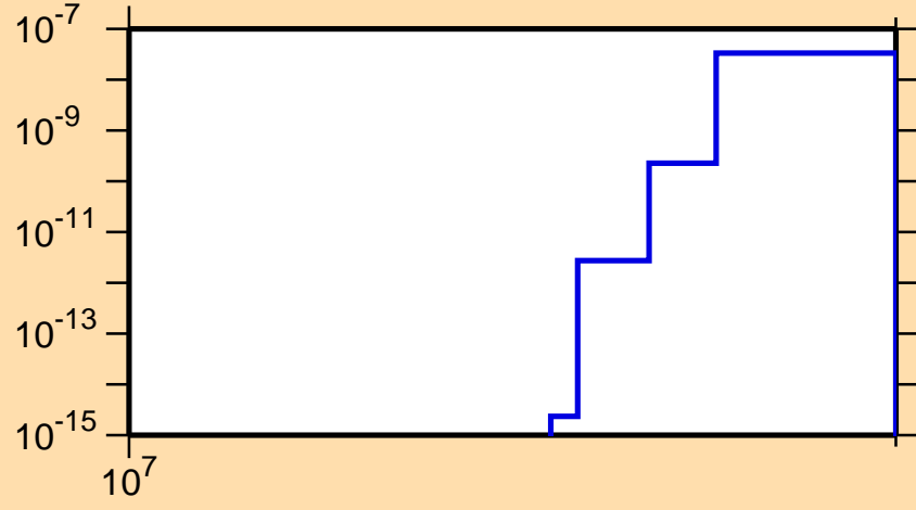
\sigma vs. E for ^{240}\text{U}(n,nd)
