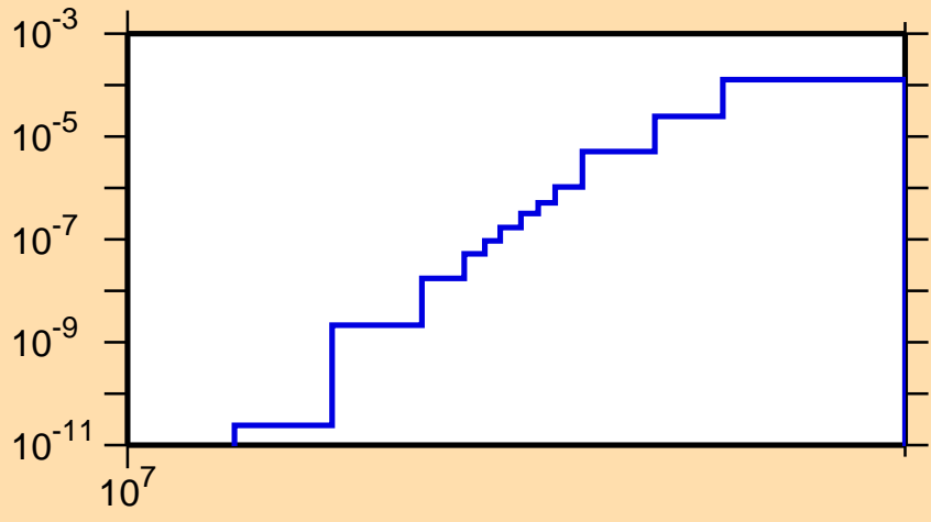
\sigma vs. E for ^{240}\text{U}(n,np)
