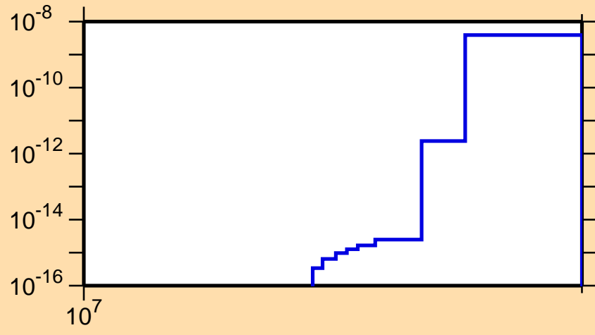
\sigma vs. E for ^{240}\text{U}(n,2np)
