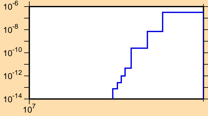
\sigma vs. E for ^{240}\text{U}(n,nt)
