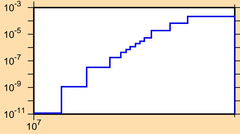
\sigma vs. E for ^{240}\text{U}(n,t)
