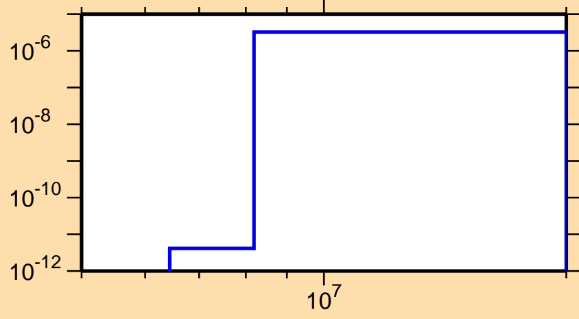
\sigma vs. E for ^{240}\text{U}(n,\alpha)
