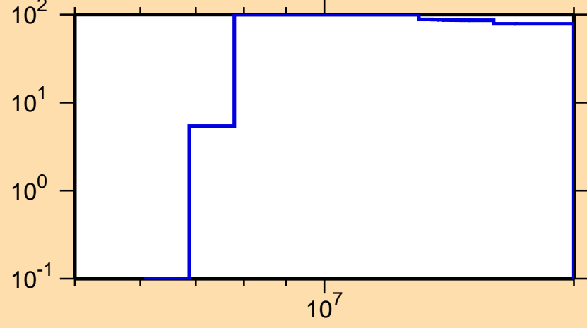
\Delta\sigma/\sigma vs. E for ^{242}\text{U}(n,p)
