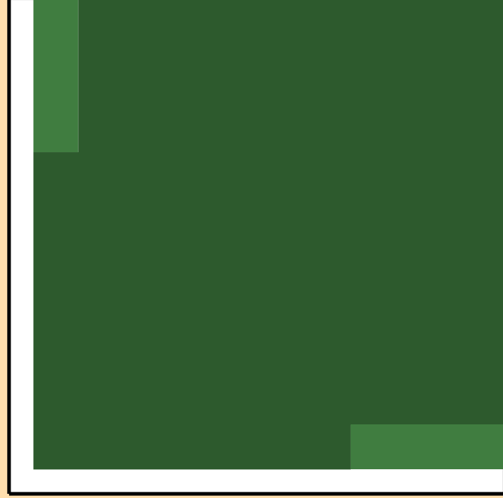
\sigma vs. E for ^{242}\text{U}(n,2n)
