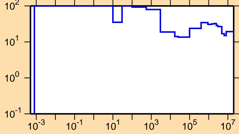
\Delta\sigma/\sigma vs. E for ^{242}\text{U}(n,\text{tot.})
