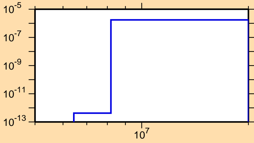
\sigma vs. E for ^{242}\text{U}(n,n\alpha)
