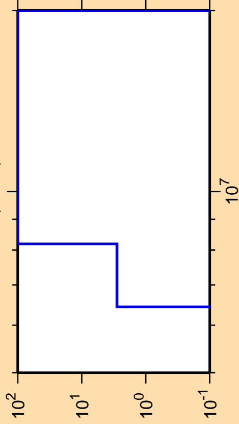
\Delta\sigma/\sigma vs. E for ^{242}\text{U}(n,n\alpha)
