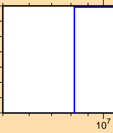
\sigma vs. E for ^{242}\text{U}(n,nt)
