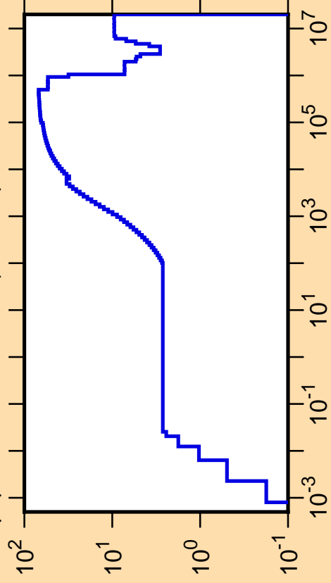
\Delta\mu/\mu vs. E for ^{151}\text{Yb}(\text{mt251})
