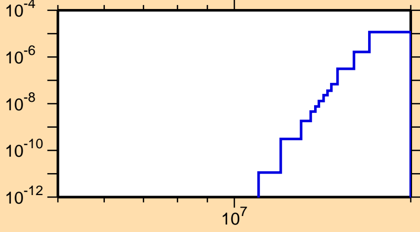
\sigma vs. E for ^{151}\text{Yb} (mt 45)
