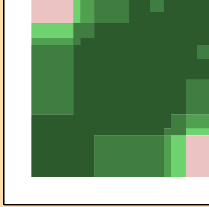
\sigma vs. E for ^{151}\text{Yb}(n,\text{inel.})
