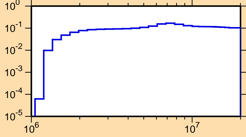
\sigma vs. E for ^{151}\text{Yb}(n,n\text{cont.})
