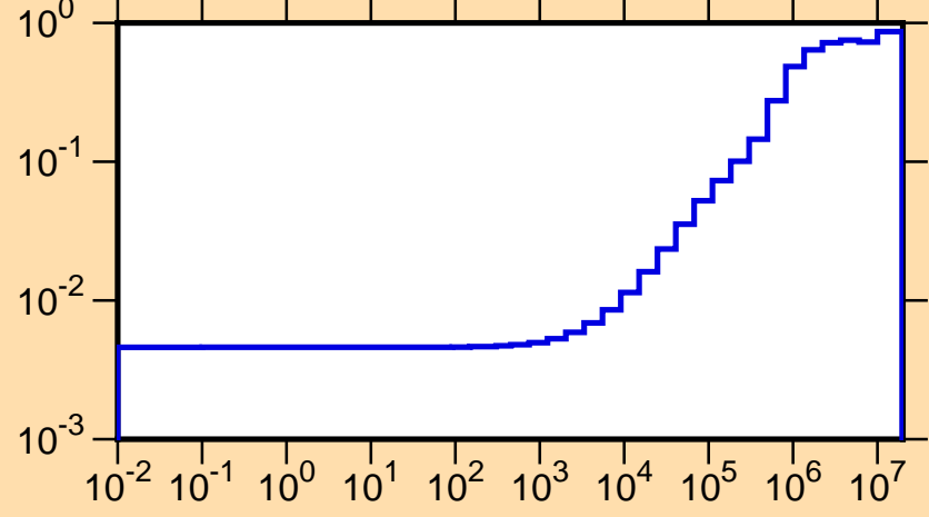
\mu vs. E for ^{151}\text{Yb}(\text{mt251})
