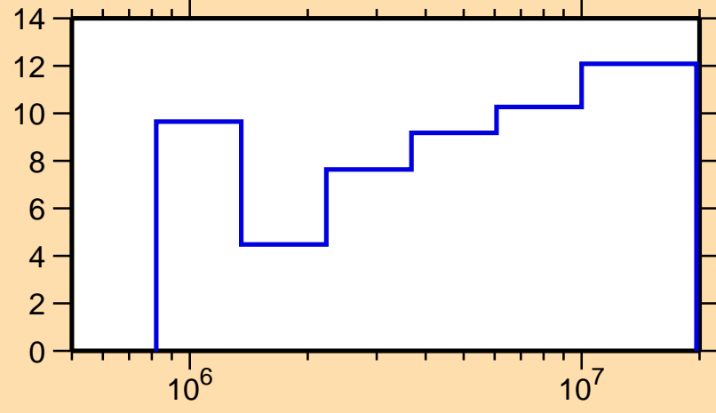
\Delta\sigma/\sigma vs. E for ^{151}\text{Yb}(n,n\text{onel.})
