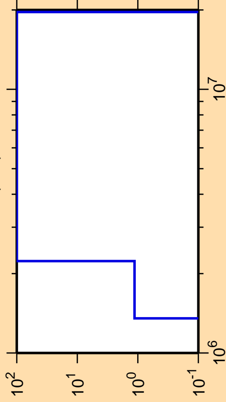
\Delta\sigma/\sigma vs. E for ^{151}\text{Yb}(n,d)
