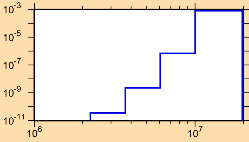
\sigma vs. E for ^{151}\text{Yb}(n,\text{He3})
