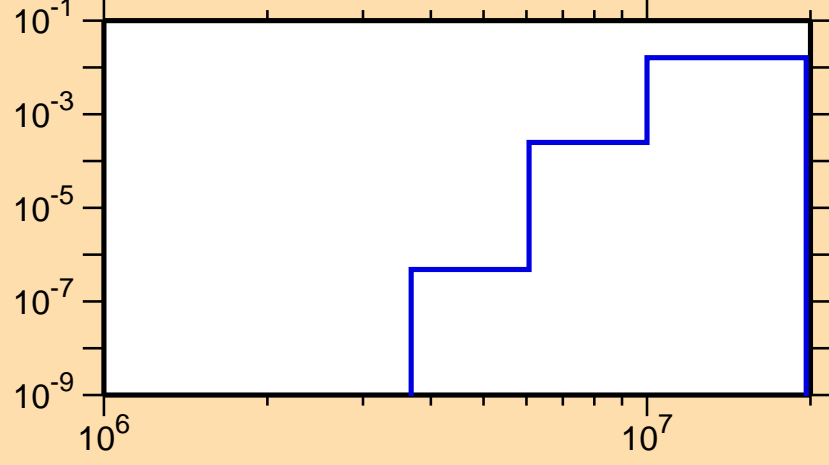
\sigma vs. E for ^{151}\text{Yb}(n,d)
