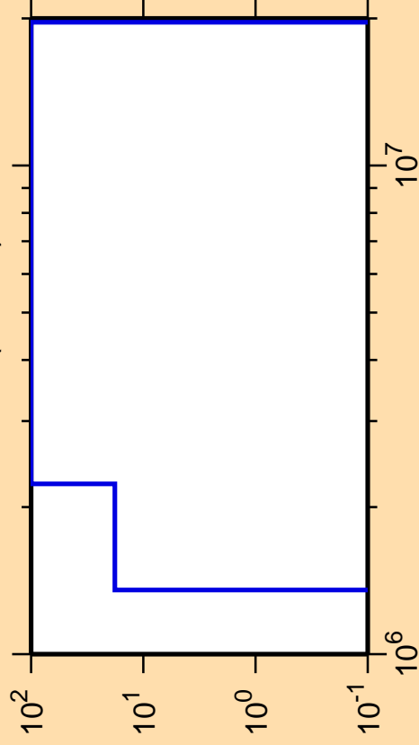
\Delta\sigma/\sigma vs. E for ^{151}\text{Yb}(n,\text{He3})
