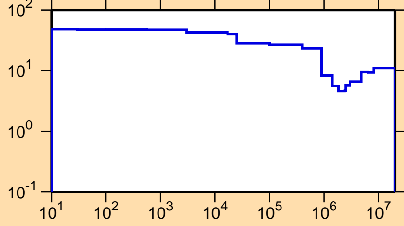
\Delta\sigma/\sigma vs. E for ^{151}\text{Yb}(n,\text{nonel.})
