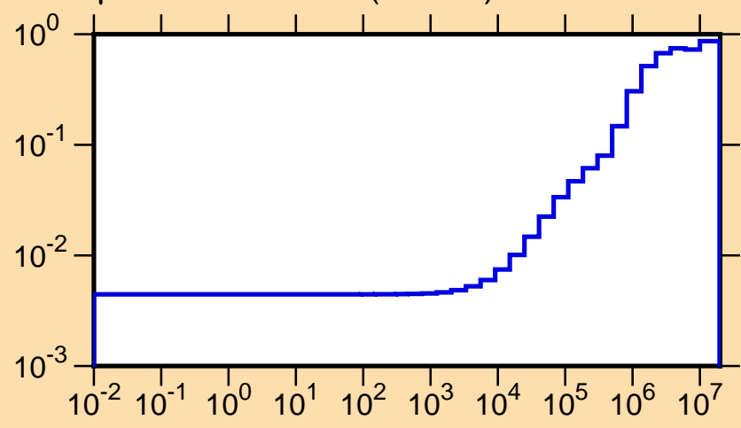
\mu vs. E for ^{152}\text{Yb}(\text{mt251})
