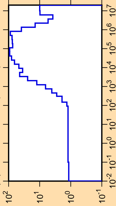
\Delta\mu/\mu vs. E for ^{152}\text{Yb}(\text{mt251})
