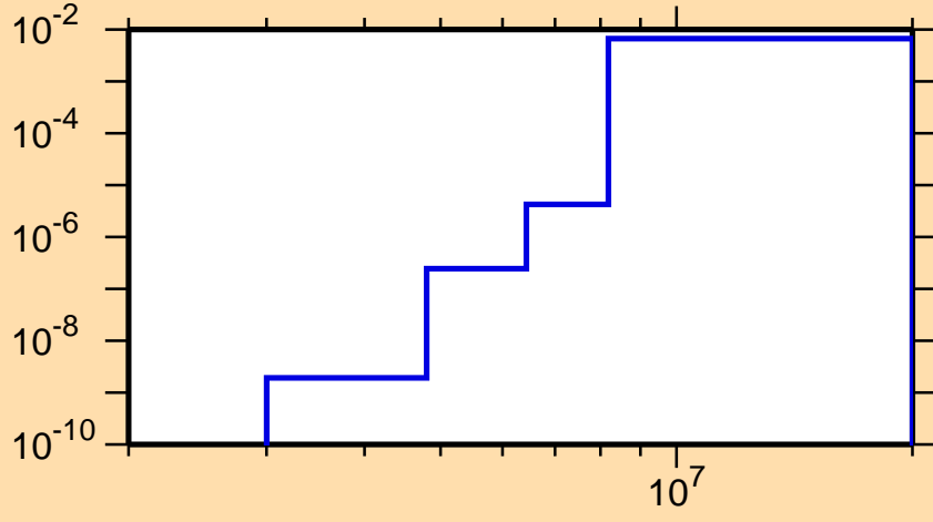
\sigma vs. E for ^{152}\text{Yb}(n,d)
