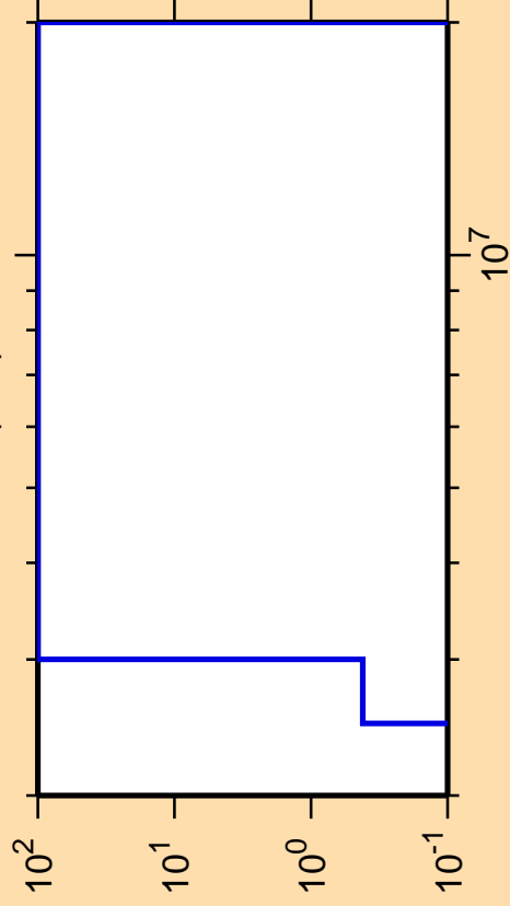
\Delta\sigma/\sigma vs. E for ^{152}\text{Yb}(n,d)
