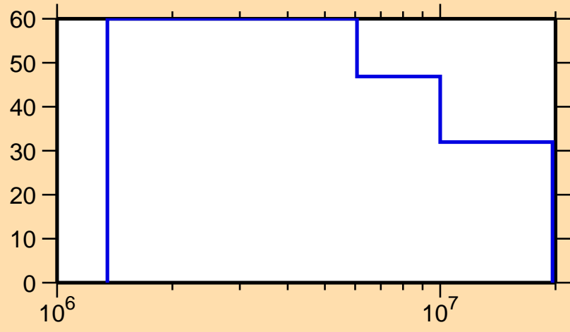
\Delta\sigma/\sigma vs. E for ^{153}\text{Yb}(n,ncont.)
