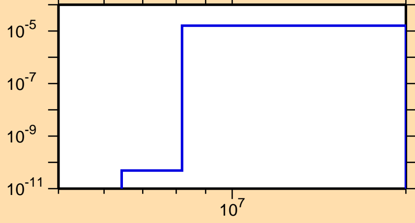
\sigma vs. E for ^{155}\text{Yb} (mt 45)
