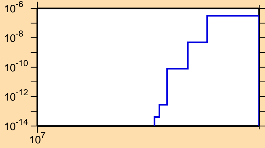
\sigma vs. E for ^{156}\text{Yb}(n,nd)
