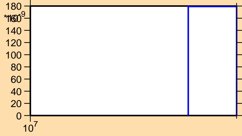
\sigma vs. E for ^{156}\text{Yb}(n,3n)
