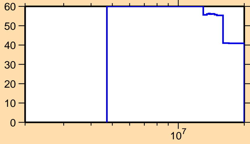
\Delta\sigma/\sigma vs. E for ^{156}\text{Yb}(n,el.)
