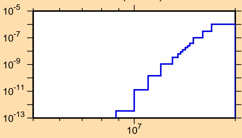
\sigma vs. E for ^{156}\text{Yb}(\text{mt117})
