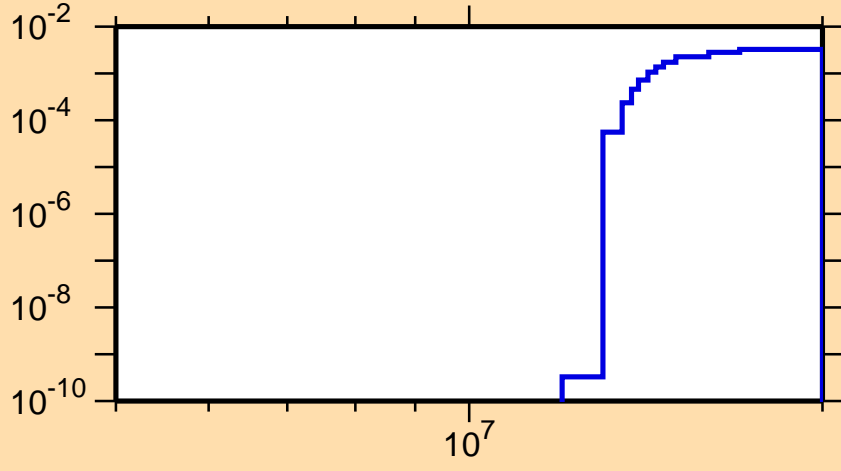
\sigma vs. E for ^{156}\text{Yb}(n,2n\alpha)
