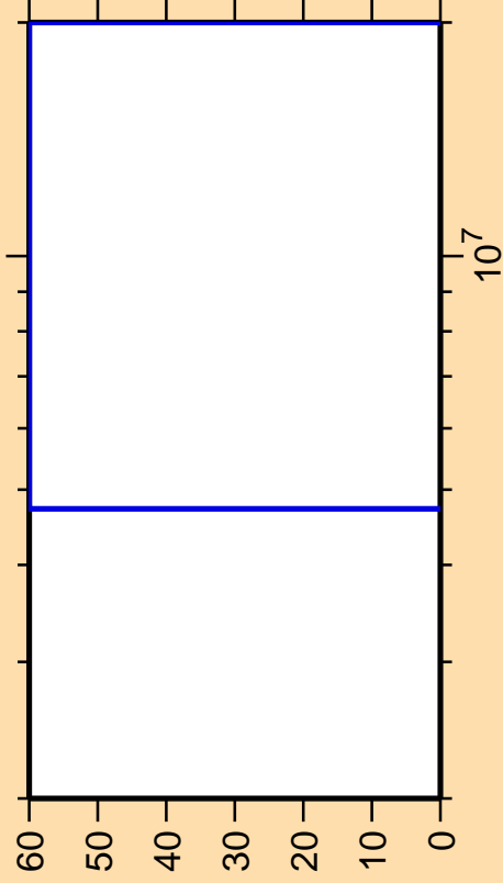
\Delta\sigma/\sigma vs. E for ^{156}\text{Yb}(n,ncont.)
