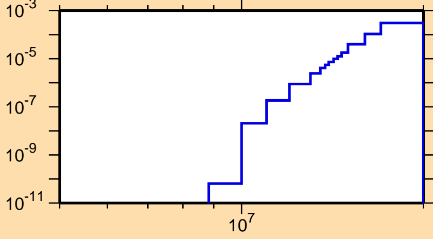
\sigma vs. E for ^{156}\text{Yb} (mt 45)
