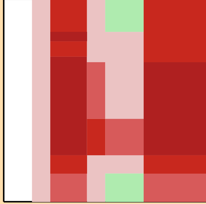
\Delta\sigma/\sigma vs. E for ^{157}\text{Yb}(n,n\text{cont.})
