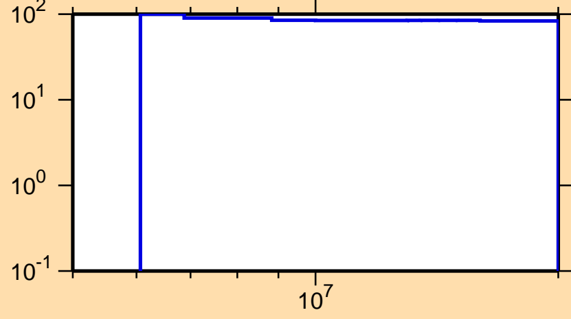
\Delta\sigma/\sigma vs. E for ^{157}\text{Yb}(n,n\text{cont.})
