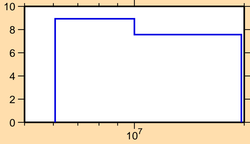
\Delta\sigma/\sigma vs. E for ^{157}\text{Yb}(n,n\text{onel.})
