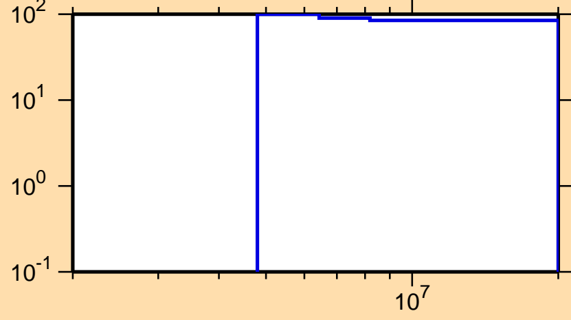
\Delta\sigma/\sigma vs. E for ^{157}\text{Yb}(n,ncont.)
