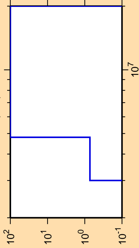
\Delta\sigma/\sigma vs. E for ^{157}\text{Yb}(n,d)
