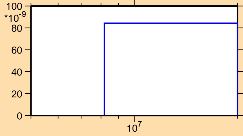
\sigma vs. E for ^{157}\text{Yb}(n,3n)
