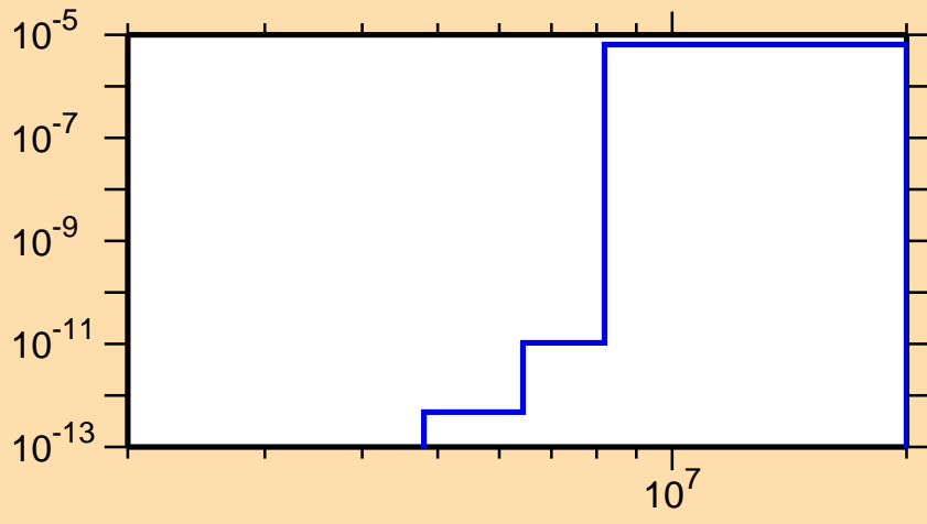
\sigma vs. E for ^{157}\text{Yb}(n,\text{He3})
