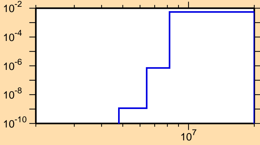
\sigma vs. E for ^{157}\text{Yb}(n,d)
