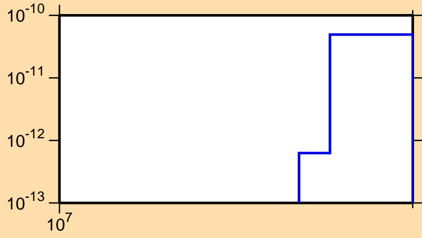
\sigma vs. E for ^{158}\text{Yb} (mt 34)
