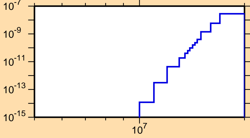
\sigma vs. E for ^{158}\text{Yb}(\text{mt117})
