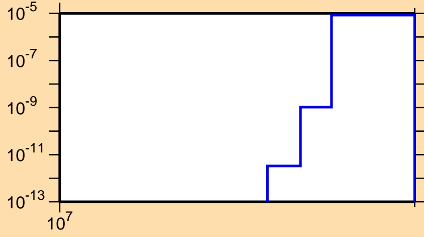
\sigma vs. E for ^{158}\text{Yb}(n,2np)
