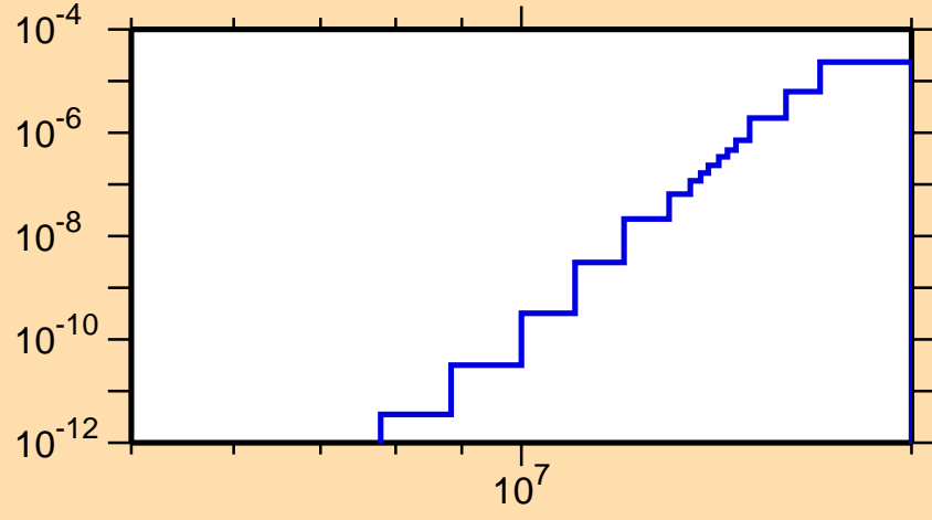
\sigma vs. E for ^{158}\text{Yb}(n,\text{He3})
