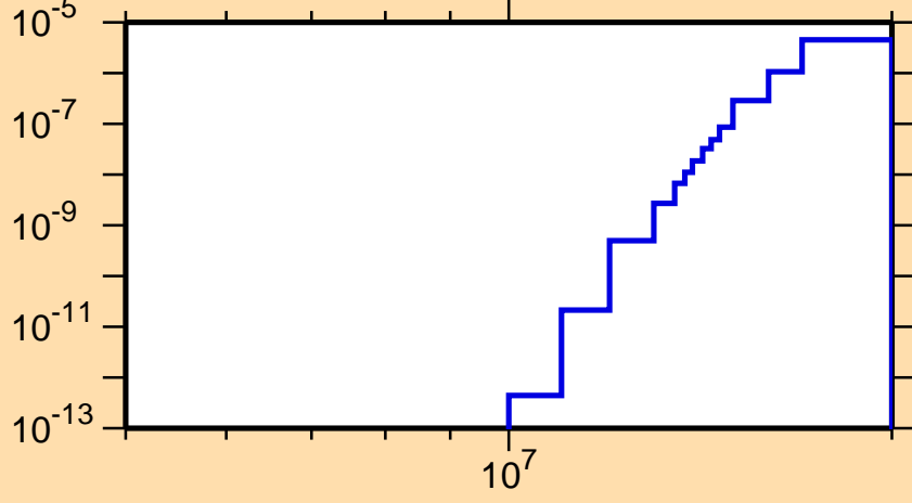
\sigma vs. E for ^{158}\text{Yb} (mt 45)
