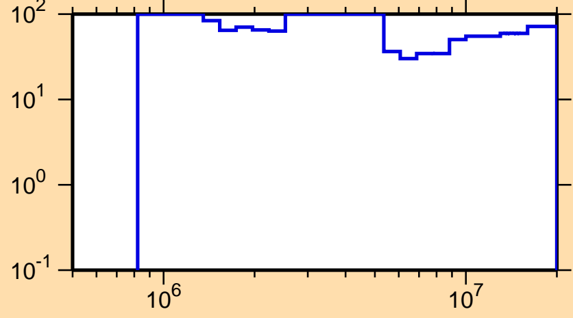
\Delta\sigma/\sigma vs. E for ^{158}\text{Yb}(n,ncont.)
