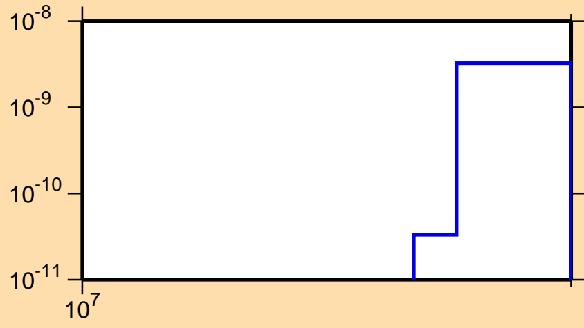
\sigma vs. E for ^{158}\text{Yb}(n,\text{pt})
