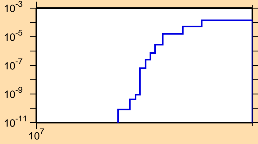
\sigma vs. E for ^{158}\text{Yb}(n,2n\alpha)
