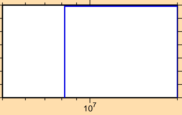
\sigma vs. E for ^{158}\text{Yb}(\text{mt117})
