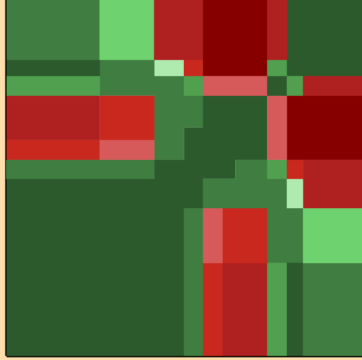
\sigma vs. E for ^{158}\text{Yb}(n,\text{inel.})
