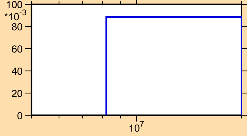
\sigma vs. E for ^{158}\text{Yb}(n,2n)
