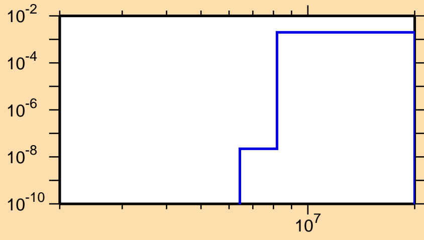
\sigma vs. E for ^{158}\text{Yb}(n,d)
