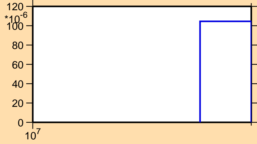
\sigma vs. E for ^{159}\text{Yb}(n,3n)
