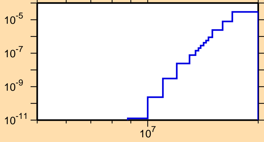
\sigma vs. E for ^{159}\text{Yb}(n,\text{He3})
