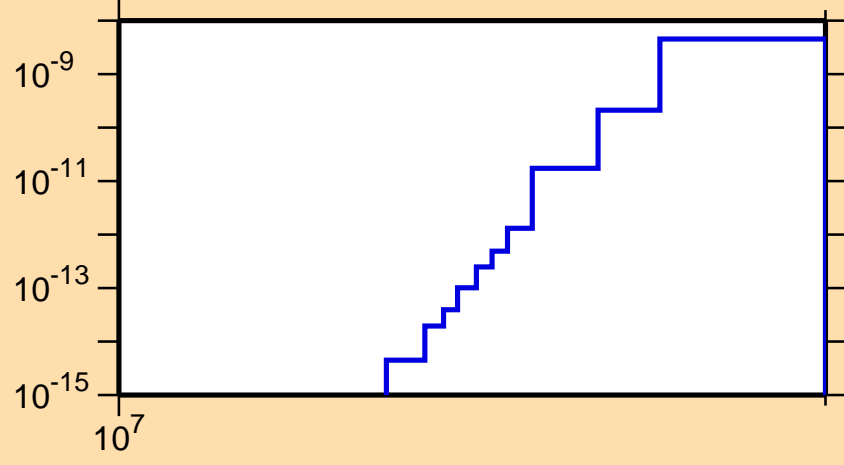
\sigma vs. E for ^{159}\text{Yb} (mt 34)
