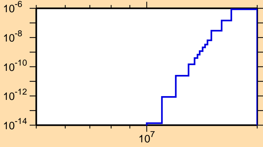
\sigma vs. E for ^{159}\text{Yb} (mt 45)
