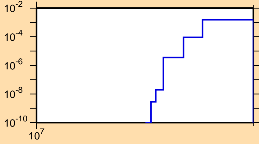
\sigma vs. E for ^{159}\text{Yb}(n,2np)
