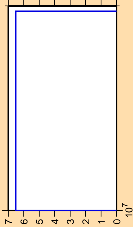
\Delta\sigma/\sigma vs. E for ^{159}\text{Yb}(n,nt)
