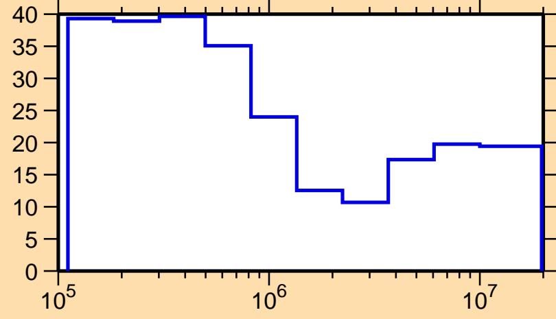
\Delta\sigma/\sigma vs. E for ^{159}\text{Yb}(n,n\text{onel.})
