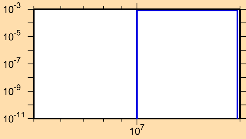
\sigma vs. E for ^{159}\text{Yb}(n,2n\alpha)
