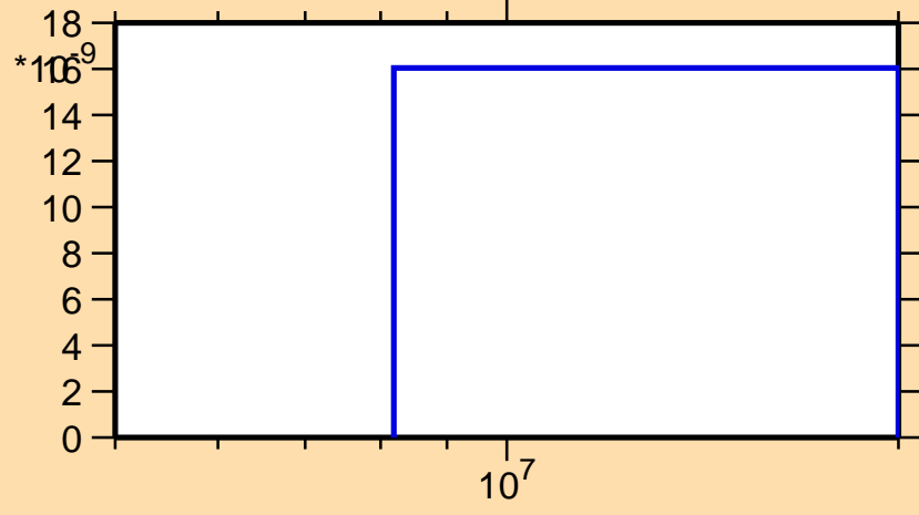
\sigma vs. E for ^{159}\text{Yb}(n,\text{pd})
