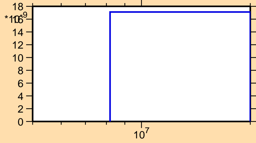
\sigma vs. E for ^{159}\text{Yb} (mt 45)
