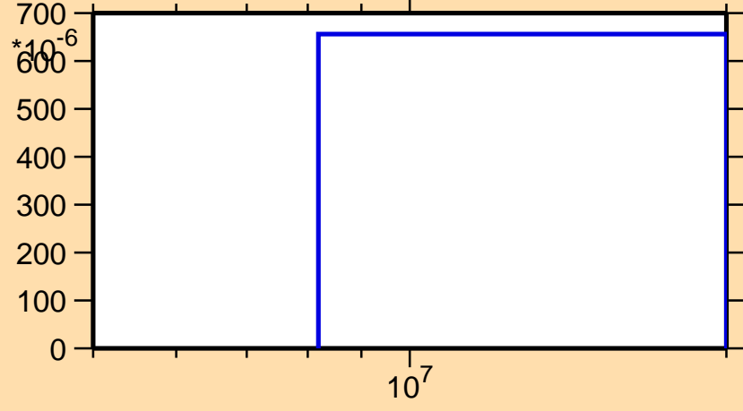
\sigma vs. E for ^{159}\text{Yb}(n,2n\alpha)
