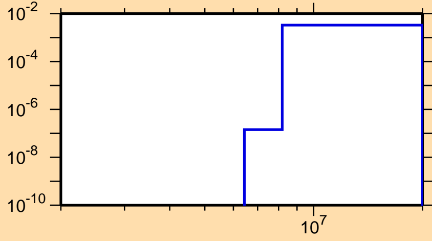
\sigma vs. E for ^{159}\text{Yb}(n,d)
