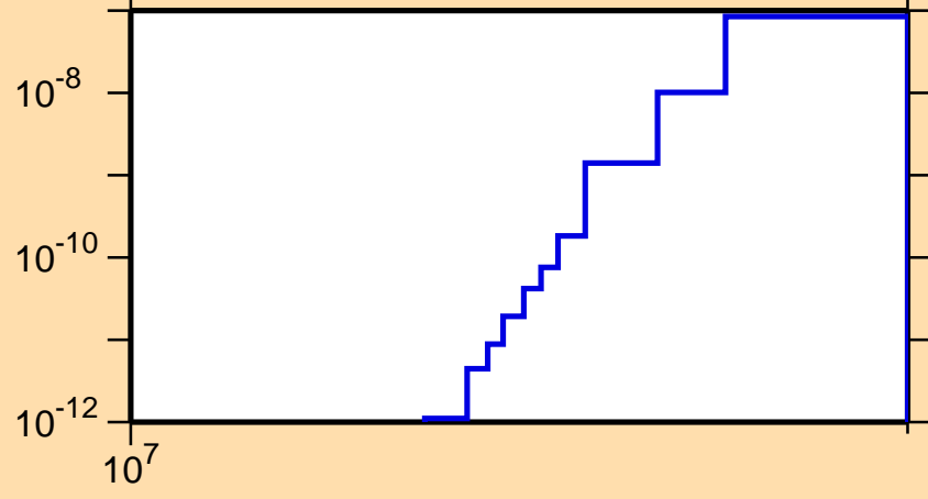
\sigma vs. E for ^{161}\text{Yb}(n,\text{pd})
