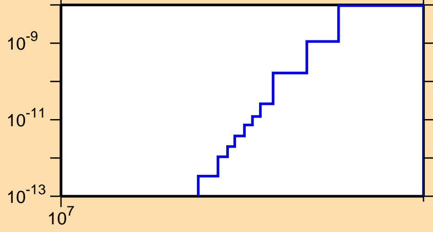
\sigma vs. E for ^{161}\text{Yb} (mt 45)
