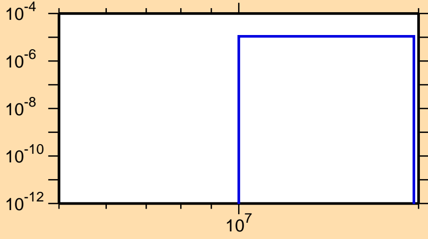
\sigma vs. E for ^{161}\text{Yb}(n,2n\alpha)
