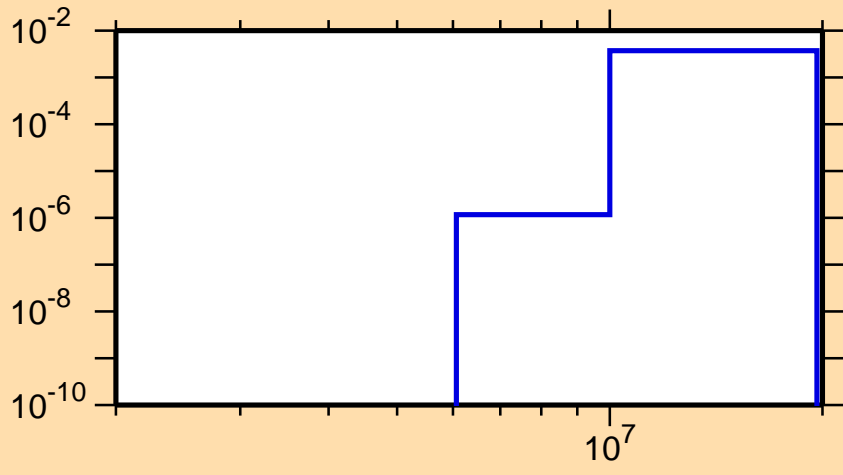
\sigma vs. E for ^{161}\text{Yb}(n,d)
