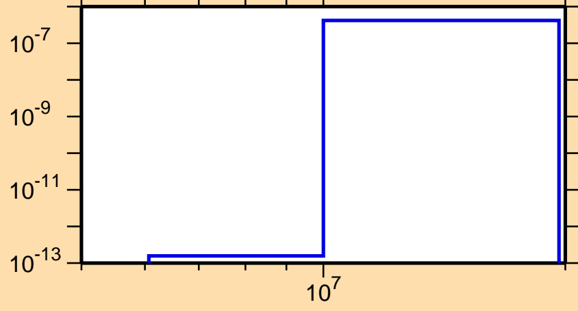
\sigma vs. E for ^{161}\text{Yb}(n,\text{He3})
