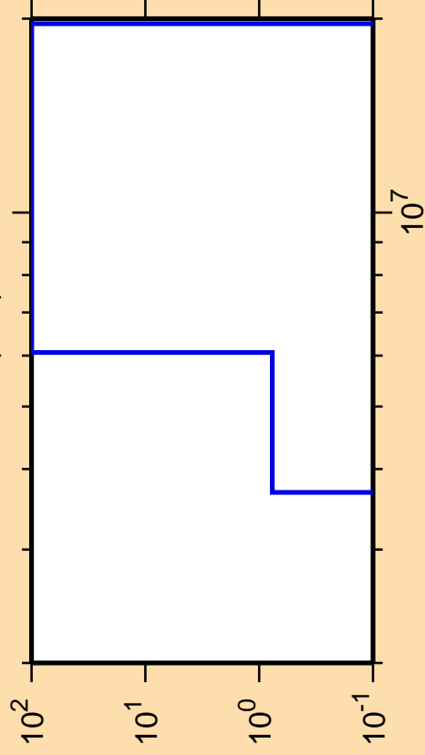
\Delta\sigma/\sigma vs. E for ^{161}\text{Yb}(n,d)
