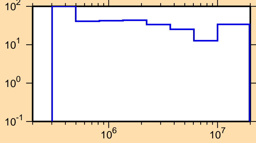
\Delta\sigma/\sigma vs. E for ^{161}\text{Yb}(n,n\text{cont.})
