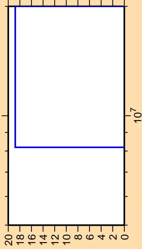
\Delta\sigma/\sigma vs. E for ^{161}\text{Yb}(n,\text{nt})
