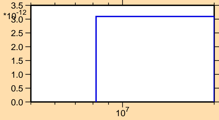
\sigma vs. E for ^{161}\text{Yb}(n,\text{nt})
