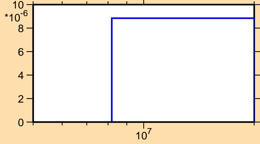
\sigma vs. E for ^{161}\text{Yb}(n,2n\alpha)
