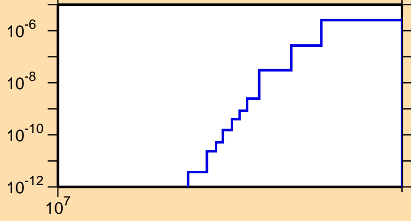
\sigma vs. E for ^{162}\text{Yb}(n,2n\alpha)
