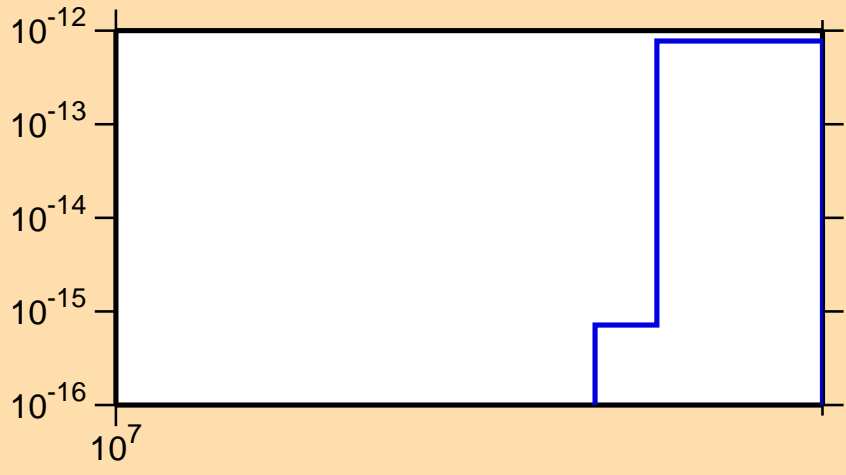
\sigma vs. E for ^{162}\text{Yb} (mt 34)
