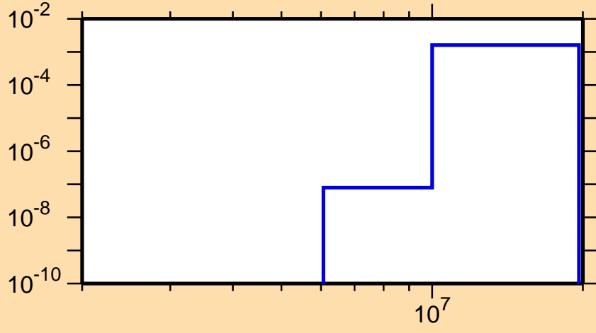
\sigma vs. E for ^{162}\text{Yb}(n,d)
