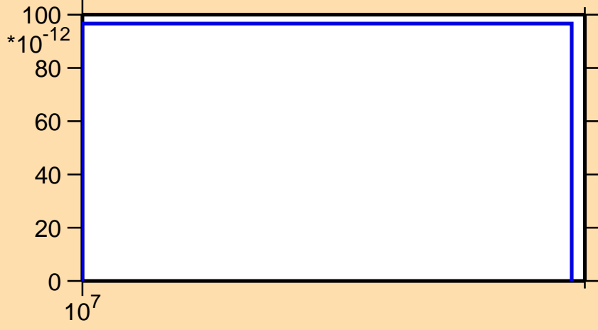
\sigma vs. E for ^{162}\text{Yb} (mt 45)
