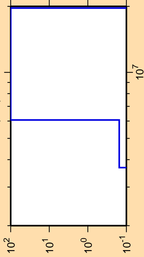
\Delta\sigma/\sigma vs. E for ^{162}\text{Yb}(n,d)
