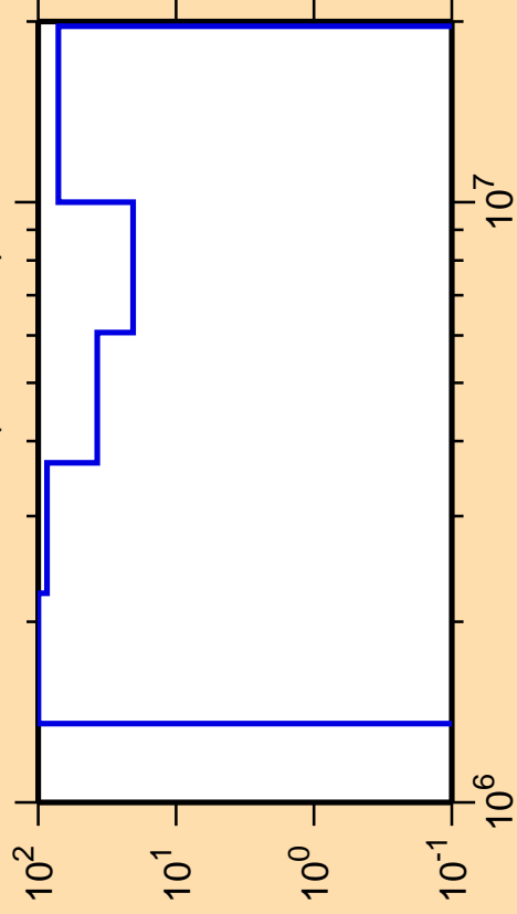
\Delta\sigma/\sigma vs. E for ^{162}\text{Yb}(n,\text{ncont.})
