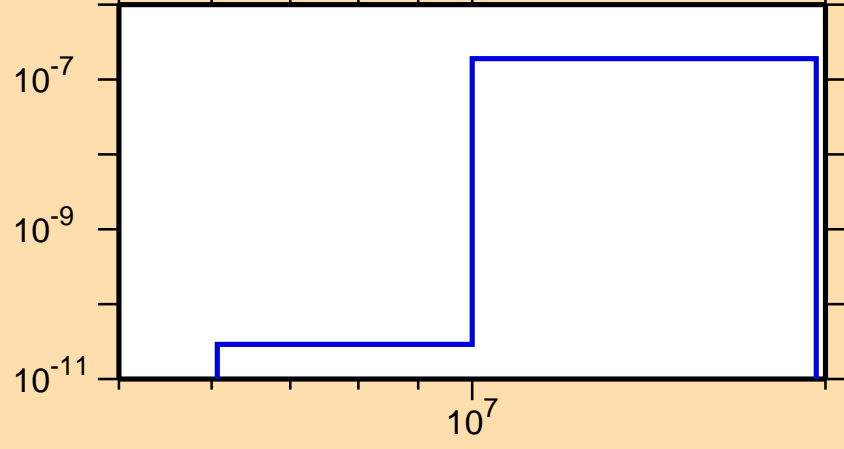
\sigma vs. E for ^{162}\text{Yb}(n,p\alpha)
