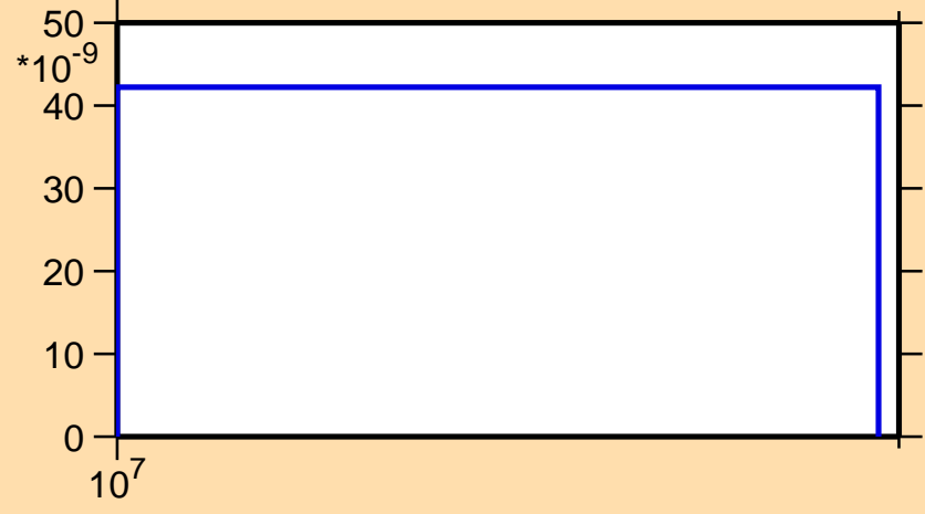
\sigma vs. E for ^{162}\text{Yb}(n,2n\alpha)
