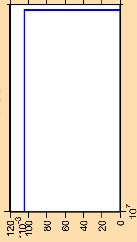
\Delta\sigma/\sigma vs. E for ^{162}\text{Yb}(n,\text{pt})
