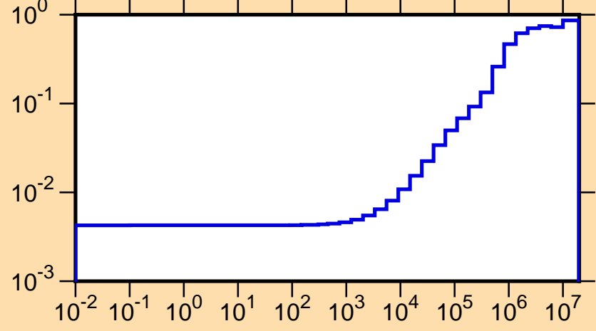
\mu vs. E for ^{163}\text{Yb}(\text{mt251})
