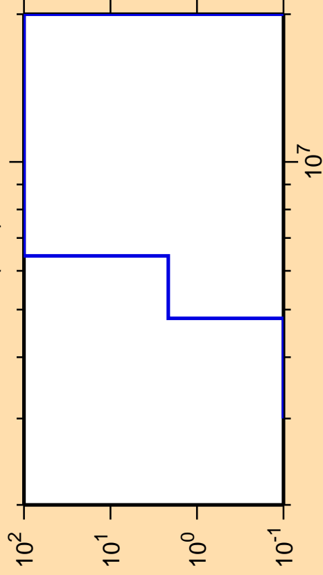
\Delta\sigma/\sigma vs. E for ^{163}\text{Yb}(n,d)
