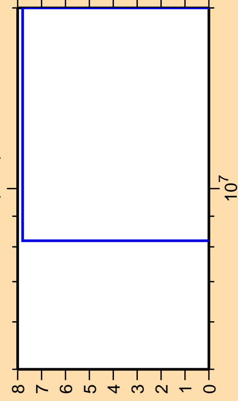
\Delta\sigma/\sigma vs. E for ^{163}\text{Yb}(n,\text{nt})
