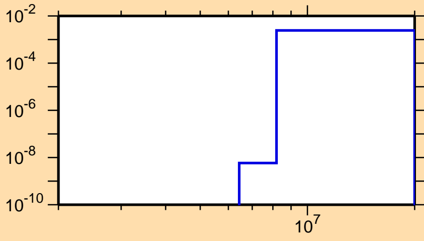
\sigma vs. E for ^{163}\text{Yb}(n,d)
