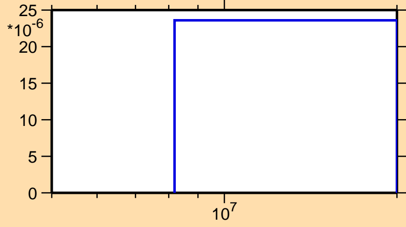
\sigma vs. E for ^{163}\text{Yb}(n,3n)
