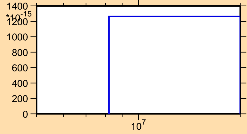
\sigma vs. E for ^{163}\text{Yb}(n,\text{nt})
