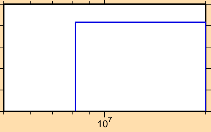
\sigma vs. E for ^{163}\text{Yb}(n,\text{He3})
