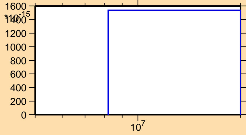
\sigma vs. E for ^{164}\text{Yb}(n,\text{nt})
