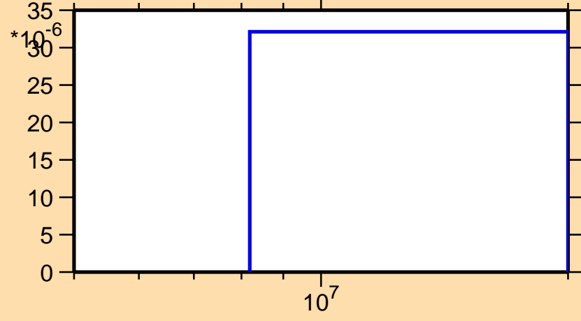
\sigma vs. E for ^{164}\text{Yb}(n,3n)
