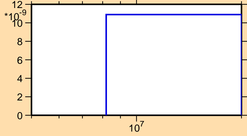
\sigma vs. E for ^{164}\text{Yb}(n,p\alpha)
