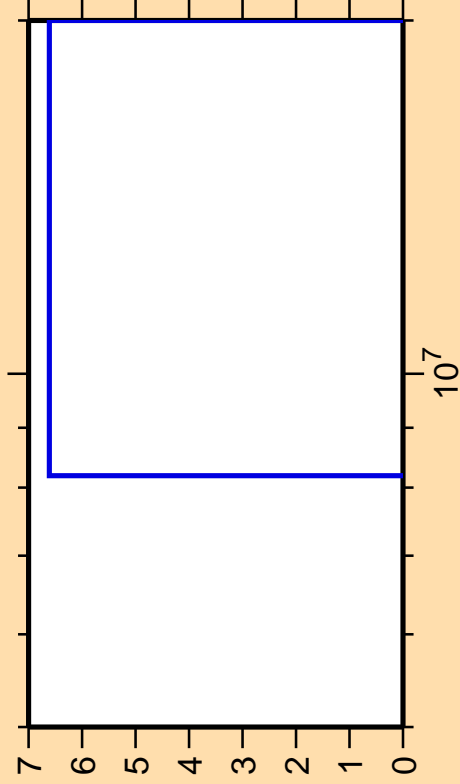
\Delta\sigma/\sigma vs. E for ^{164}\text{Yb}(n,\text{nt})
