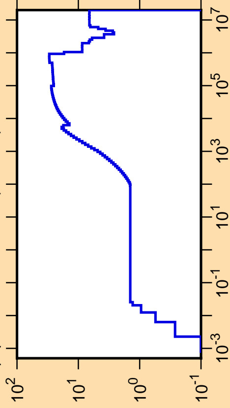
\Delta\mu/\mu vs. E for ^{165}\text{Yb}(\text{mt251})
