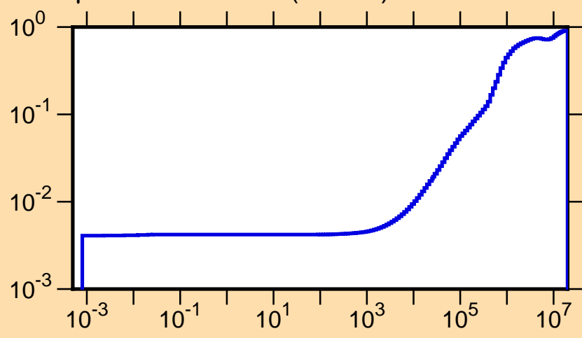
\mu vs. E for ^{165}\text{Yb}(\text{mt251})
