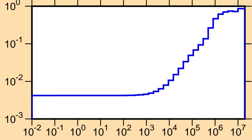
\mu vs. E for ^{165}\text{Yb}(\text{mt251})
