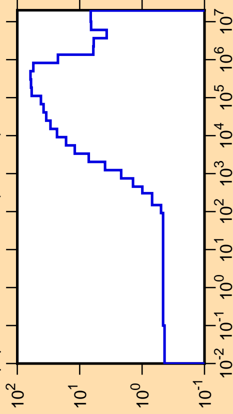
\Delta\mu/\mu vs. E for ^{166}\text{Yb}(\text{mt251})
