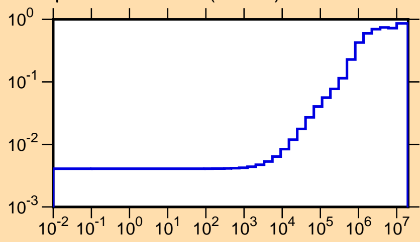
\mu vs. E for ^{166}\text{Yb}(\text{mt251})
