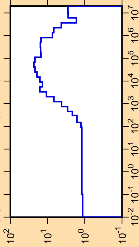
\Delta\mu/\mu vs. E for ^{167}\text{Yb}(\text{mt251})
