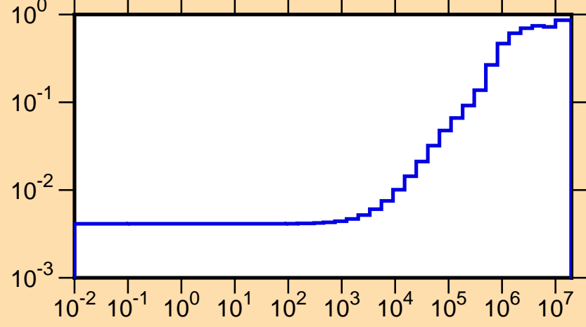
\mu vs. E for ^{167}\text{Yb}(\text{mt251})
