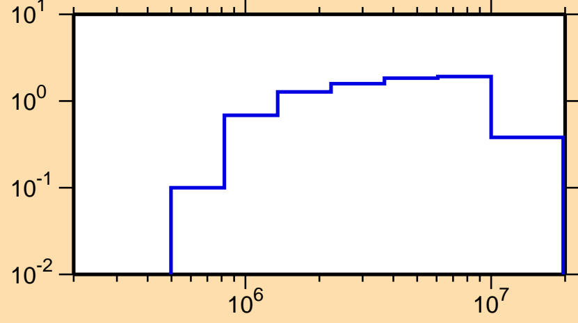
\sigma vs. E for ^{167}\text{Yb}(n,n\text{cont.})
