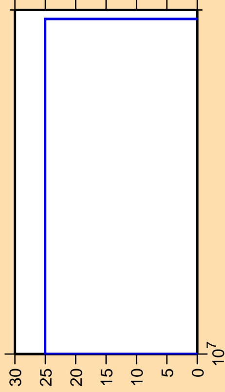
\Delta\sigma/\sigma vs. E for ^{167}\text{Yb}(n,\text{nt})
