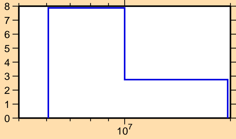
\Delta\sigma/\sigma vs. E for ^{167}\text{Yb}(n,2n)
