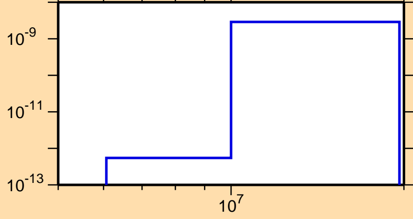
\sigma vs. E for ^{167}\text{Yb}(n,p\alpha)
